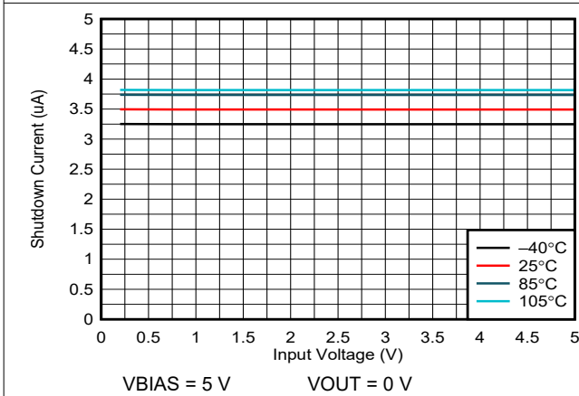
图 6-4. VBIAS Shutdown Current vs Input Voltage
