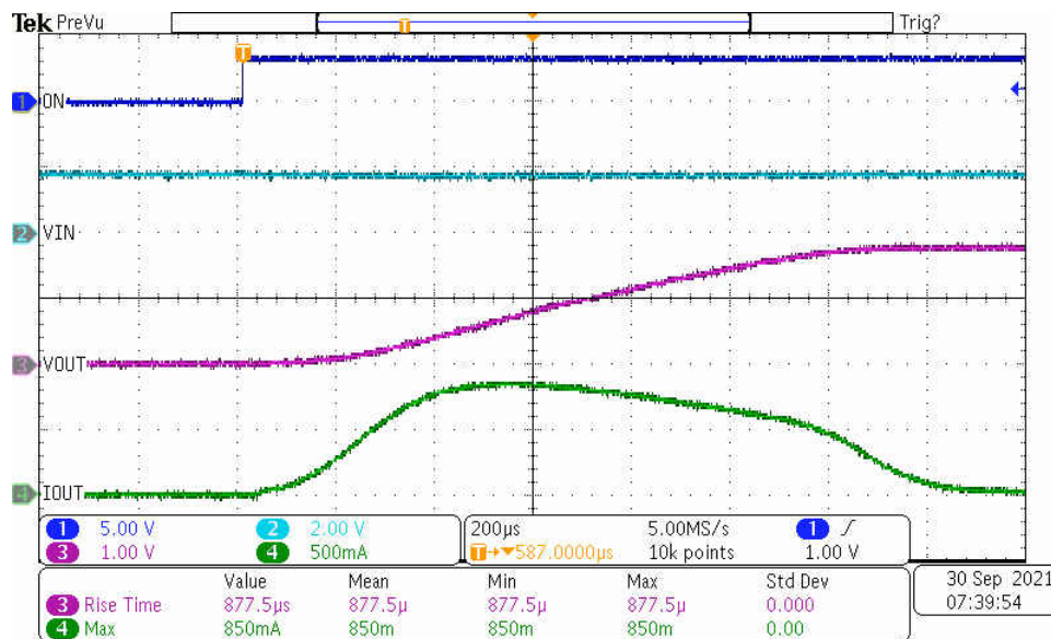
图 8-2. TPS22998 Turn-On into 470 \mu\text{F} ( C_T = V_{\text{BIAS}} )
