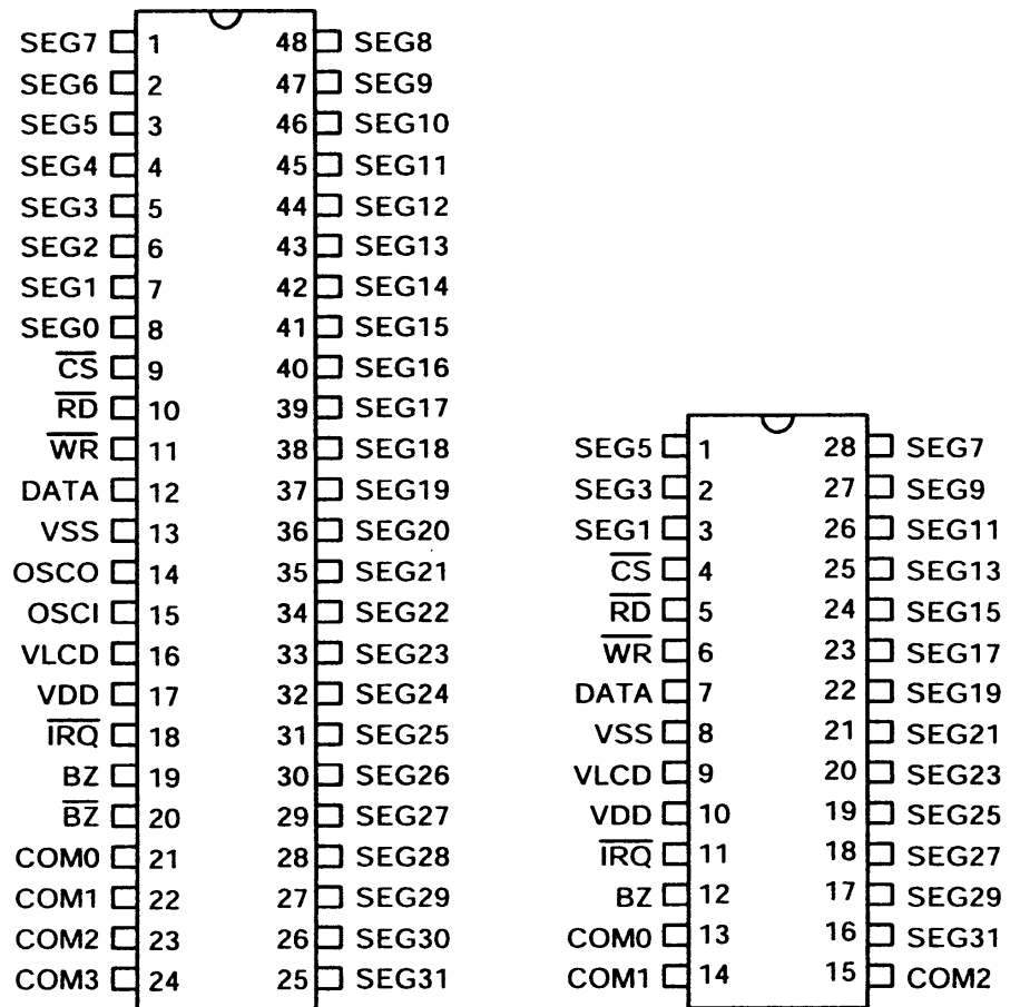
48 SSOP/PDIP
